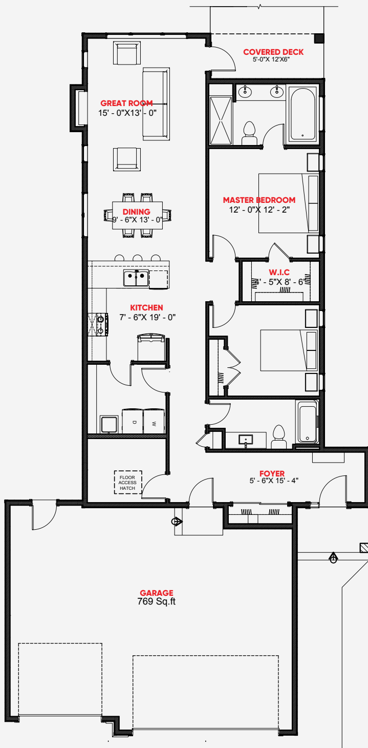
MAIN FLOOR PLAN 1,350 sq.ft.
